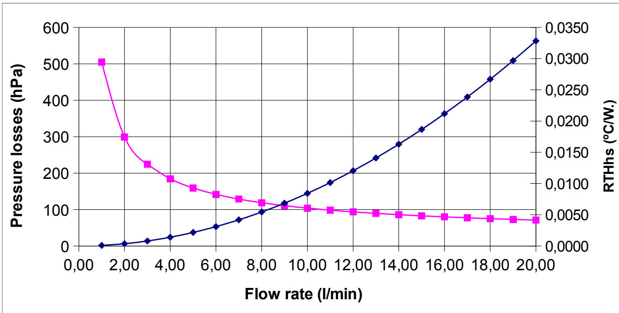
RTHhsw with H2O/Glicol 50%
