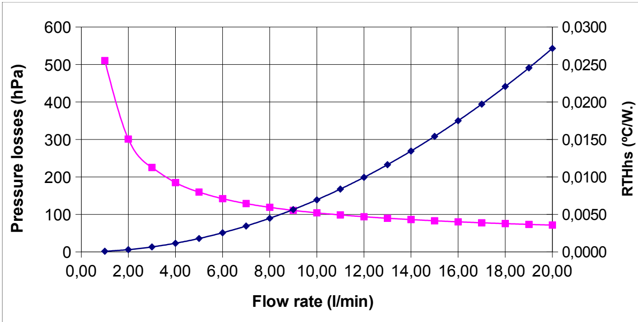
RTHhsw an pressure losses with H2O/Glicol 30%
