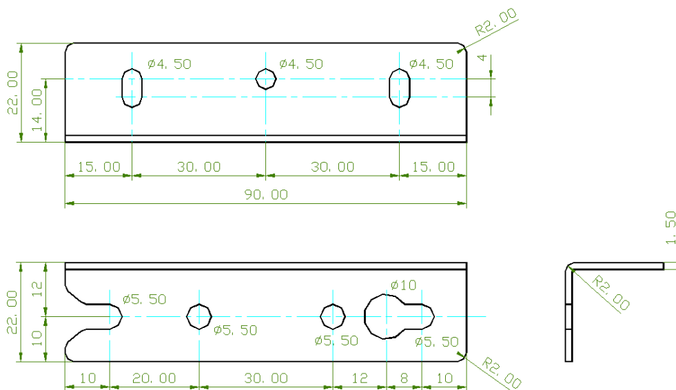
Right type (MF2Dx) illustration. All dimensions in mm
