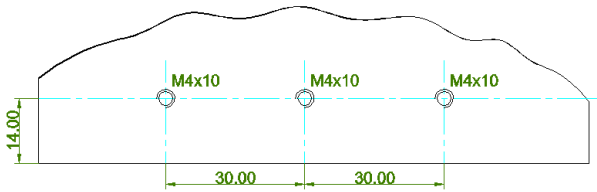
For 3 holes machining
