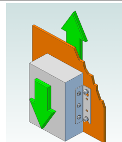
Standard test load application
