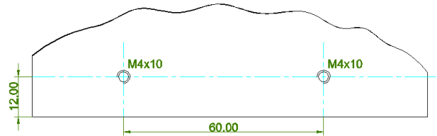
For 2 holes machining
