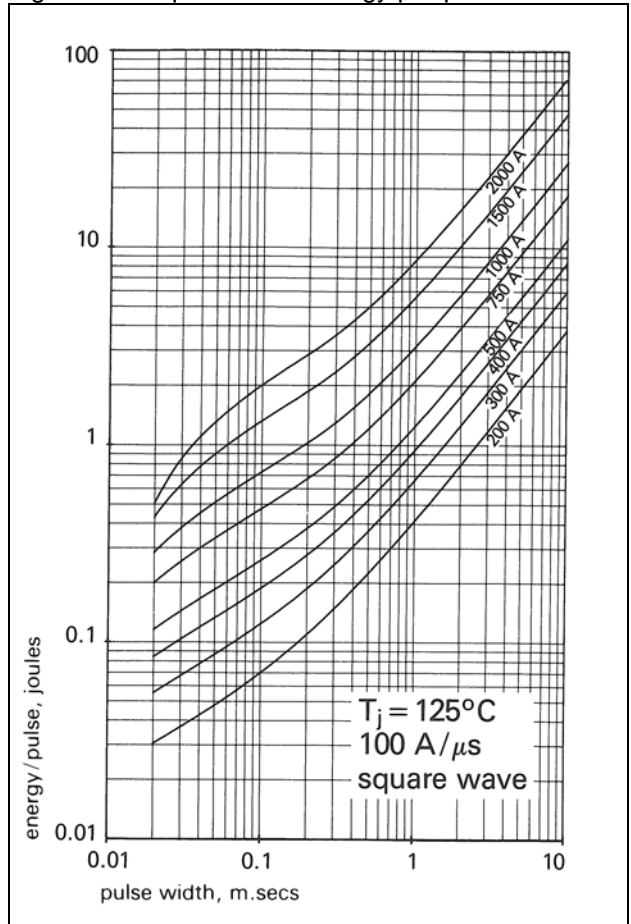
Figure 15 - Maximum reverse recovery energy loss per pulse at T_j = 125^\circ\text{C} and V_{rrm} = 804 volts
